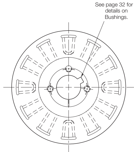
Armature View
