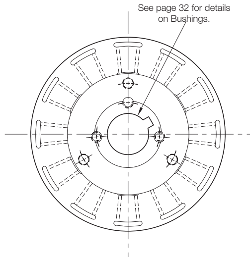
Armature View
